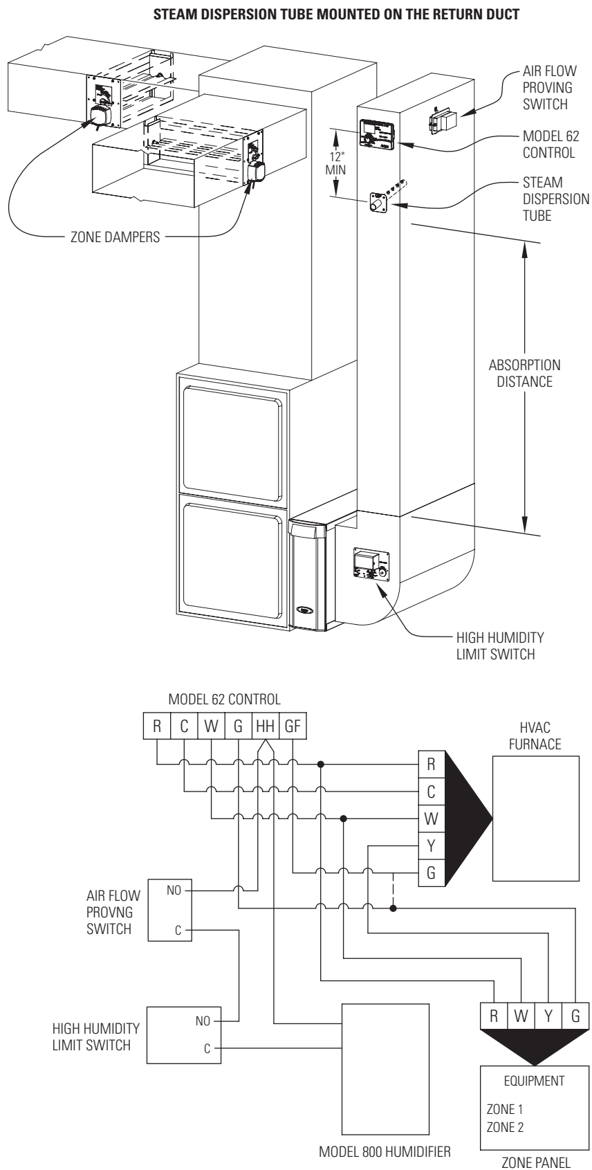
FIGURE 14 – Steam Humidifier Installed on a Zoned HVAC System
