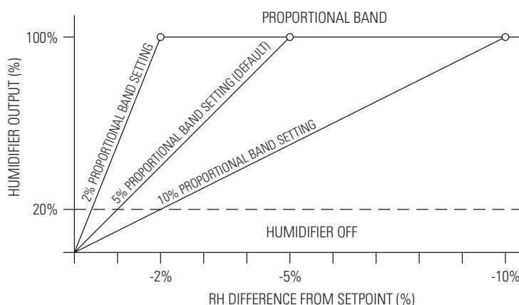
FIGURE 2 – Humidifier Output for ADCM Signal
