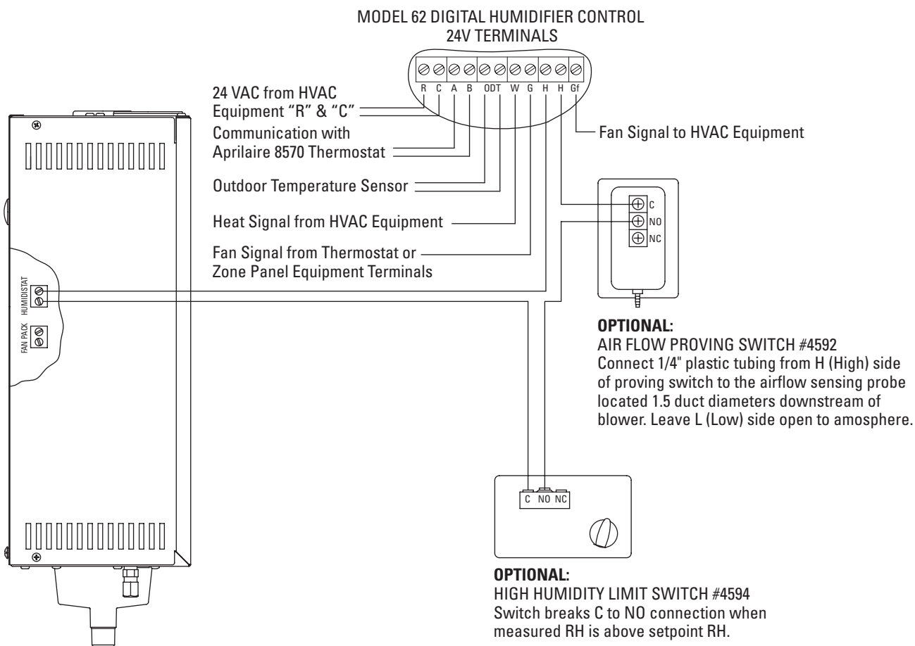
FIGURE 13 – Steam Humidifier Accessory Wiring
