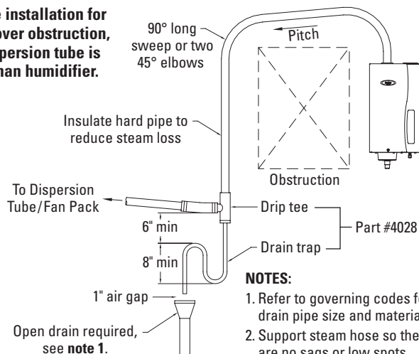
FIGURE 5 – Dispersion Tube Mounted Below Humidifier
