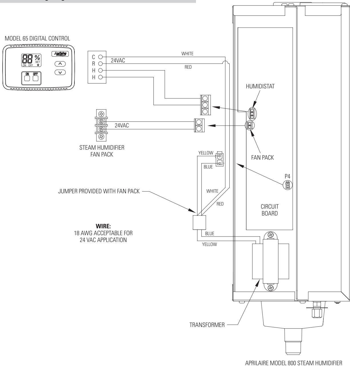
FIGURE 15 – Wiring Diagram for Manual Humidistat and Fan Pack
