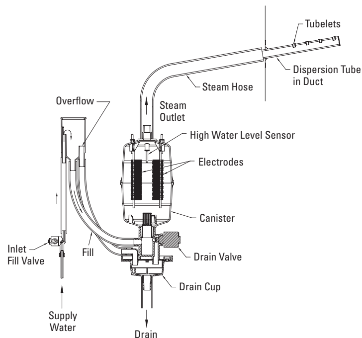
FIGURE 1 – Fill and Drain System and Canister
