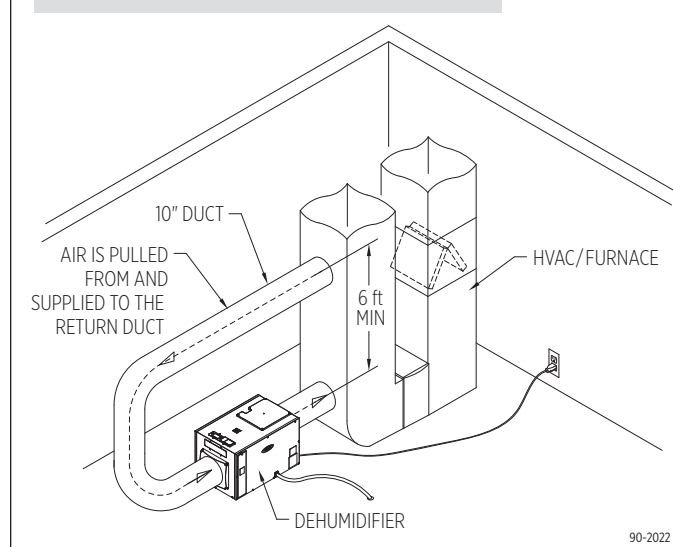
FIGURE 9 – PREFERRED BASEMENT INSTALLATION
