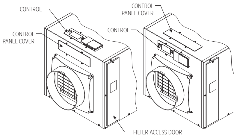
FIGURE 8 – CONTROL LOCATION
