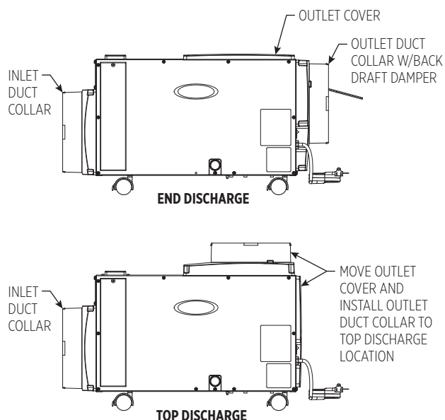
FIGURE 7 – FULLY DUCTED INSTALLATIONS
