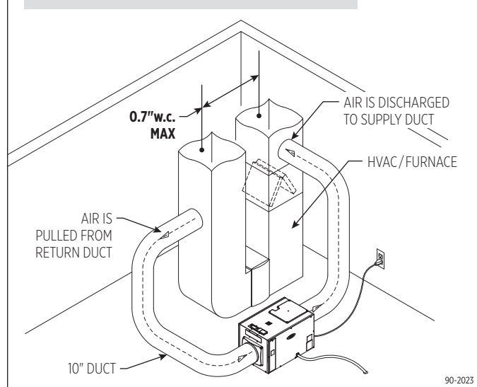
FIGURE 10 – ALTERNATE BASEMENT INSTALLATION
