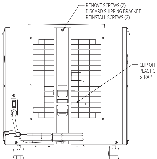
FIGURE 1 – REMOVE SHIPPING BRACKET
